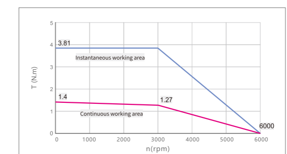
SMC60S-0040-30□□K-5LSU
