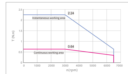
SMG60S-0020-30□□K-5LSQ
